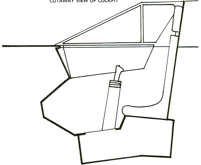
CUTAWAY VIEW OF COCKPIT
